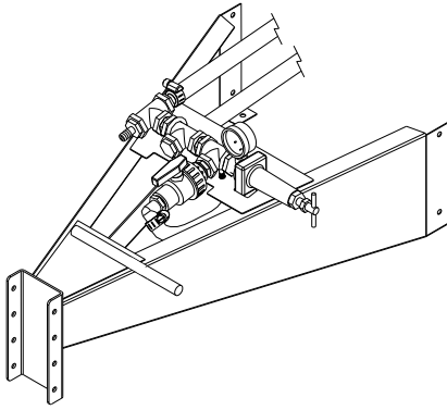
Tongue Assembly
