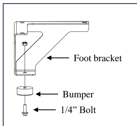
Foot bracket assembly (Qty 2)
