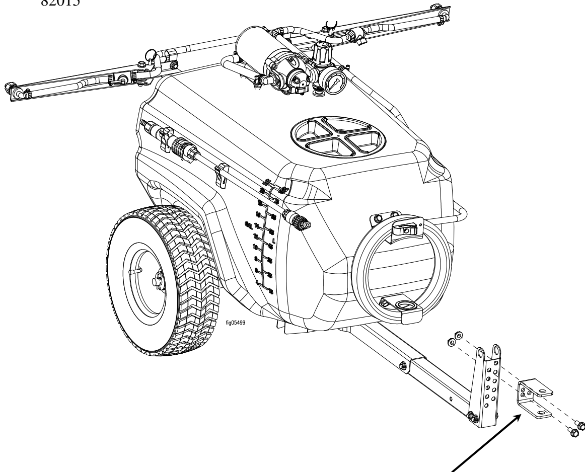
Hitch bracket
