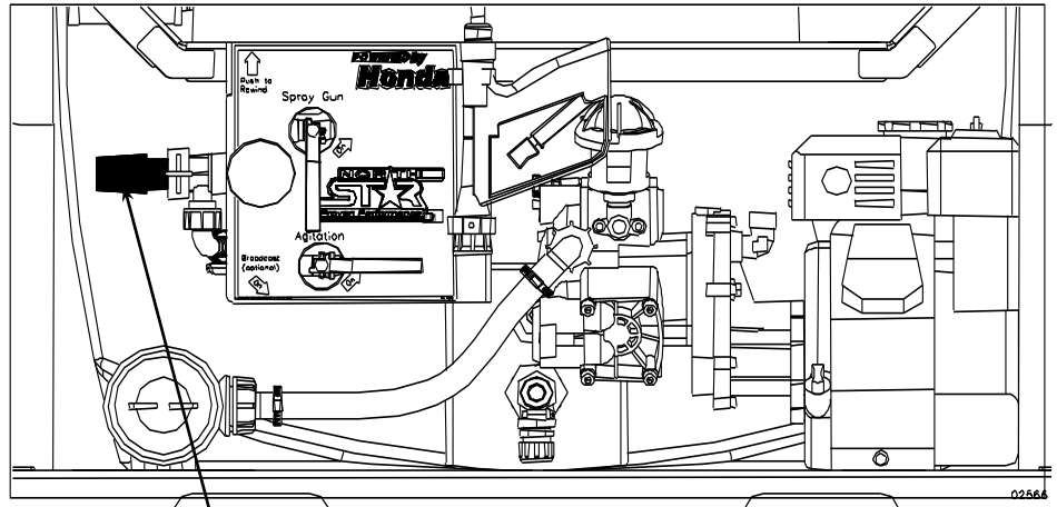
Pressure regulator
