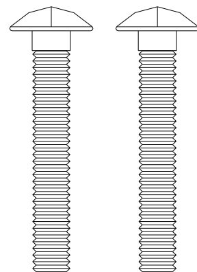
PART# 82233 BOLT, CARRIAGE GR5Z 5/16-18X2" QTY 2 (ALL MODELS)
