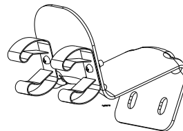
Upper Hose Wrap Bracket – Qty 1 792890: Hose Wrap Bracket – Qty 1 82059: #10-24 x 1/2" Screw – Qty 2 82065: #10-24 Lock Nut – Qty 2 777358: Gun Clip – Qty 2
